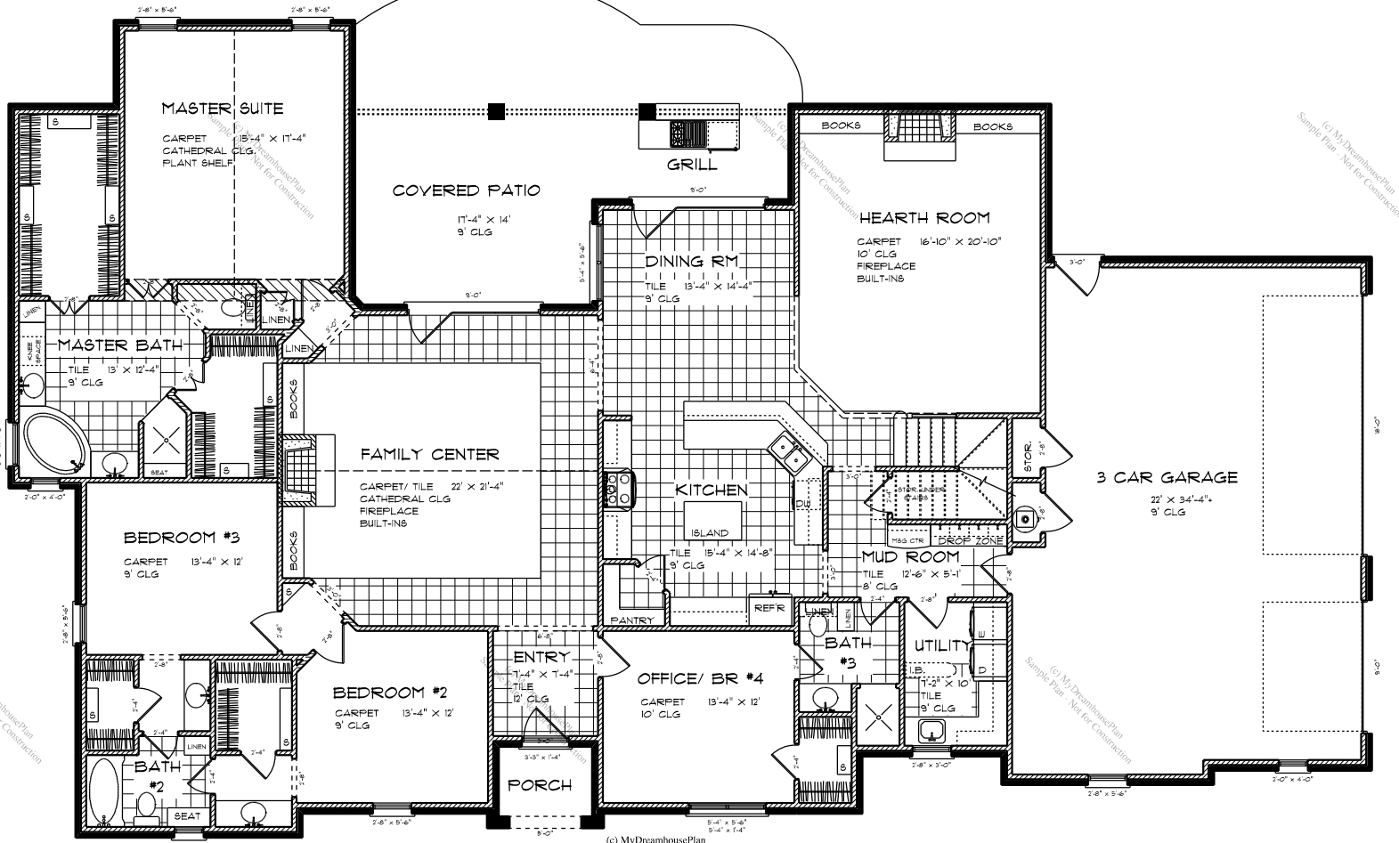
(c) MyDreamhousePlan Sample Plan - Not for Construction
